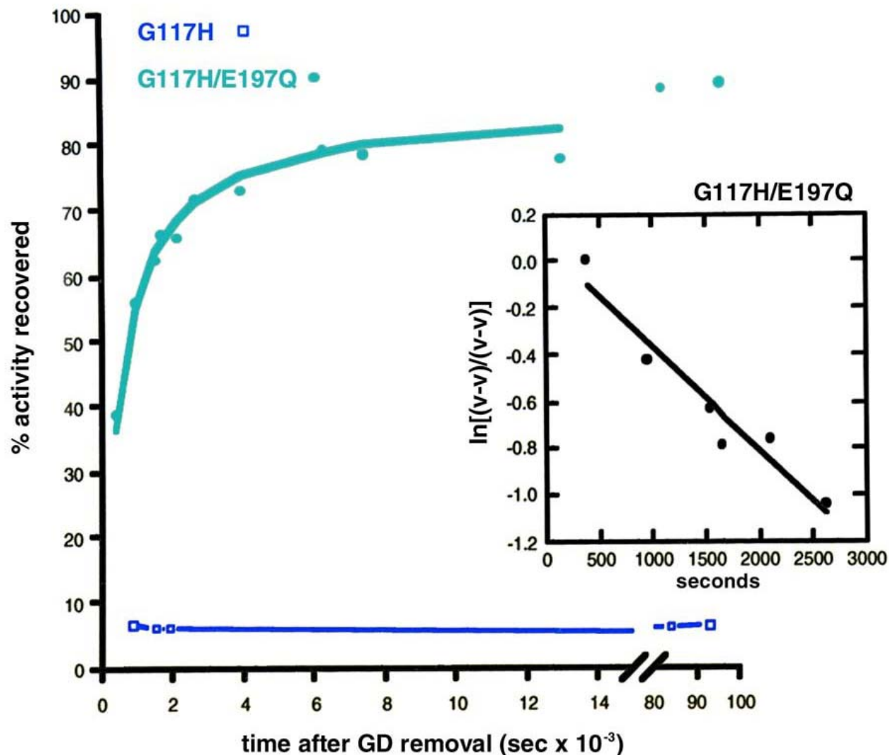
Figure B-3: Comparative Reactivation Kinetics of Soman-Inhibited Human Butyrylcholinesterase Single Mutant G117H (□) and Double Mutant G117H/E197Q (●).
