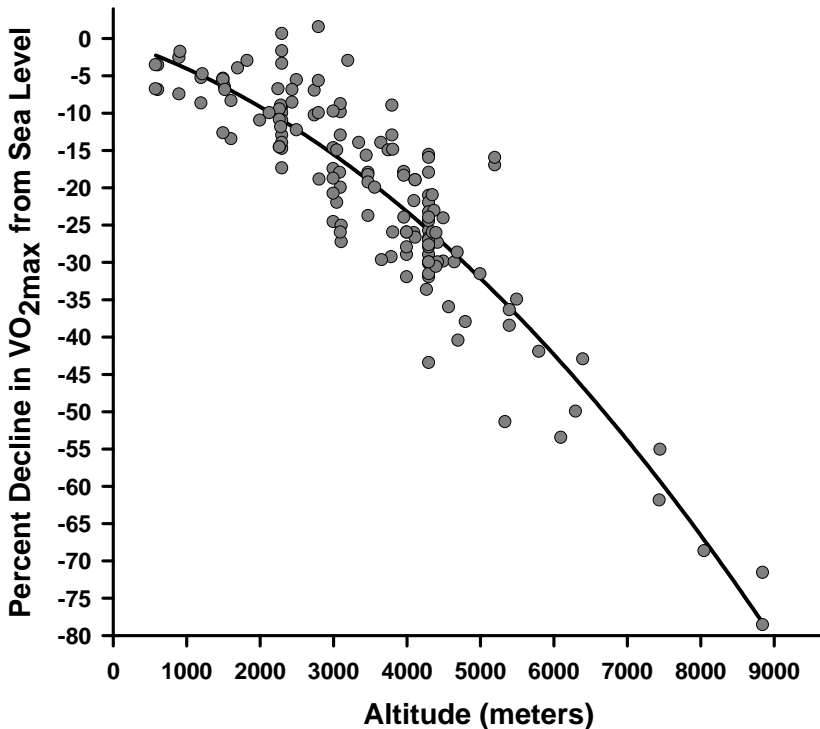
Figure 4–1. Relationship between increasing elevation and decline in maximal oxygen uptake
